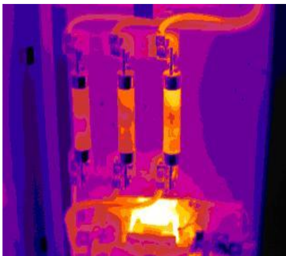
Iron palette of fuse bus bar
