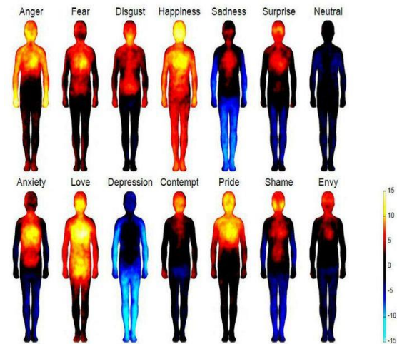
Fig. 2. Bodily topography of basic (Upper) and nonbasic (Lower) emotions associated with words. The body maps show regions whose activation increased (warm colors) or decreased (cool colors) when feeling each emotion. ( P < 0.05 FDR corrected; t > 1.94 ). The colorbar indicates the z-statistic range.
